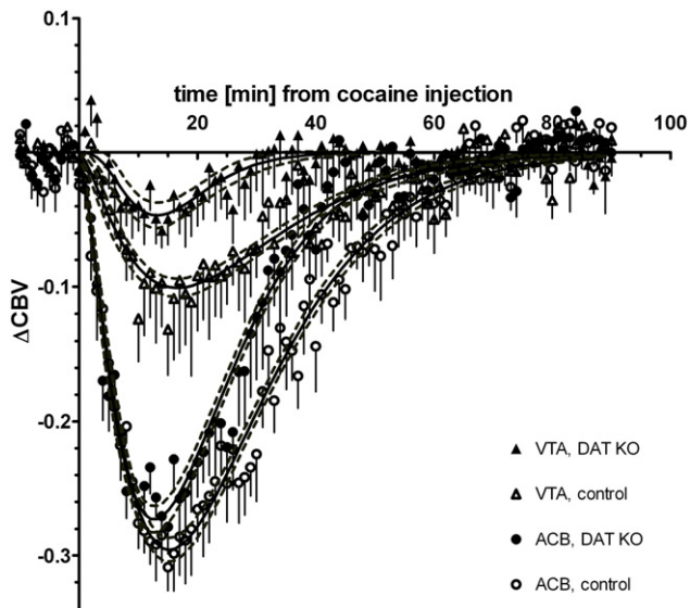
Fig. 3. \Delta\text{CBV} response in two cerebral structures (nucleus accumbens and ventral tegmental area) to an IP injection of 30 mg/kg cocaine at t = 0 . The error bars represent SEM; N = 6 DAT KO and N = 6 wild-type mice. The continuous black lines are the best gamma variate fit with the 95% confidence interval shown as dashed gray lines.
