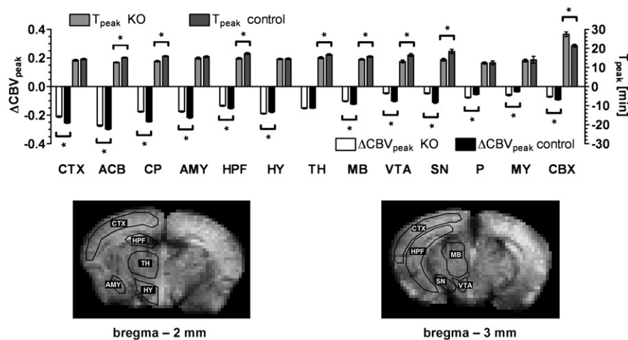
Fig. 4. Quantitative analysis of the regional CBV change after cocaine injection. Peak amplitude and the time to peak of the gamma variate fit to the signal time course are shown for specific brain regions. The error bars indicate the standard error of the mean ( N = 6 per group). In all ROIs, there is a statistically significant difference ( P < 0.01 ) between DAT KO and wild-type mice in at least one of the three fitting parameters (the shape factor \alpha is not shown). The overall time course of the \Delta CBV response is statistically different for KO and control mice in all ROIs except the thalamus. Typical ROI outlines are shown on two coronal brain slices: prefrontal, frontal, and frontoparietal cortex (CTX); nucleus accumbens (ACB); caudate putamen (CP); amygdala (AMY); hippocampal formation (HPF); thalamic nuclei (TH); hypothalamus (HY); midbrain (MB); ventral tegmental area (VTA); substantia nigra (SN); pons (P); medulla (MY); and cerebellum (CBX).
