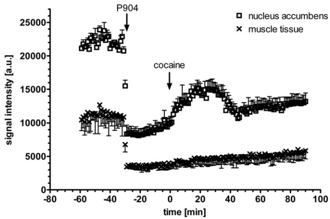
Fig. 2. Effect of IP cocaine on the signal time course in cerebral (nucleus accumbens, open symbols) and in extra-cerebral tissue (muscle, closed symbols). Injection of 25 mg/kg P904 IV at t = -30 min (left arrow) yields a 62.5% signal drop in nucleus accumbens ( 4.06 \text{ mm}^3 ) and 69.1% signal drop in muscle ( 9.58 \text{ mm}^3 ) at TE = 9.5 ms. The second arrow indicates the IP injection of cocaine (30 mg/kg), which leads to a signal increase in the cerebral tissue corresponding to a CBV decrease. The error bars show the standard deviation of the signal within the ROI in a single mouse. This is a typical signal time course prior to detrending.
